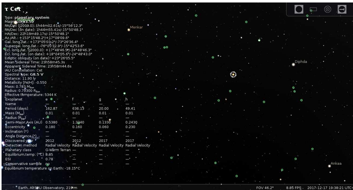
Figure 14.4: Planetary system \tau Ceti
