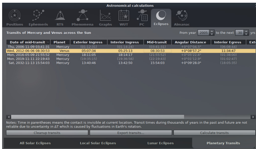
Figure 4.45: Astronomical Calculations (AstroCalc): Eclipses / Planetary Transits
