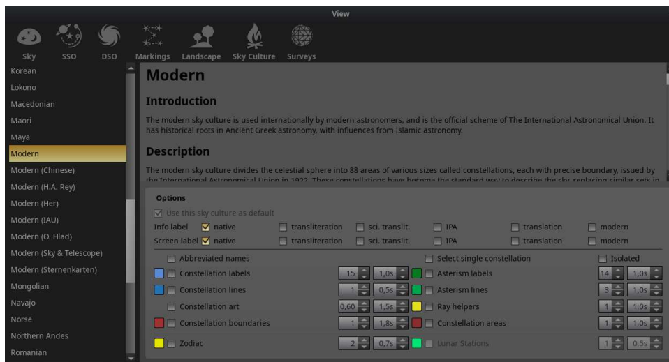
Figure 4.16: View Settings Window: Sky Culture Tab
